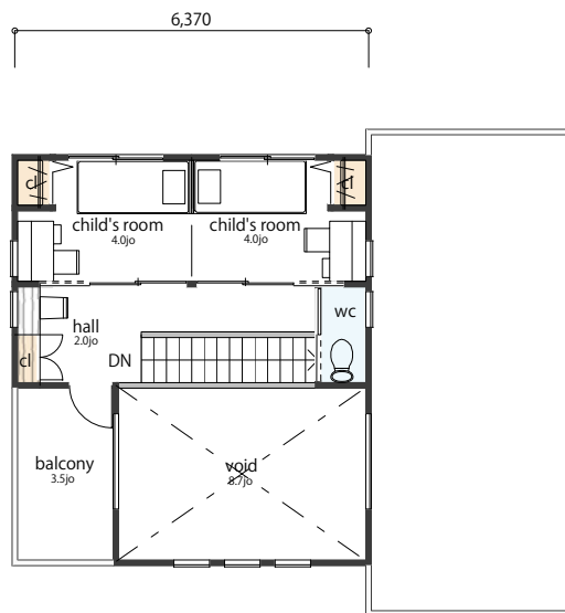
FLOOR PLAN 2F
