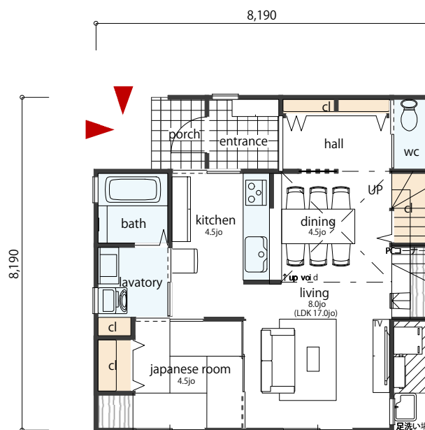
FLOOR PLAN 1F
