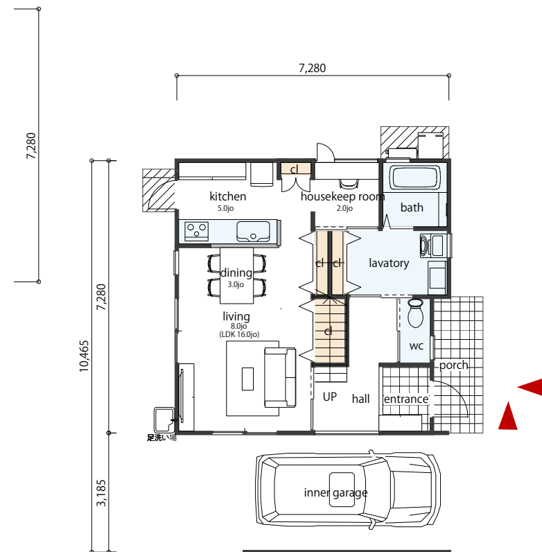
FLOOR PLAN 1F
