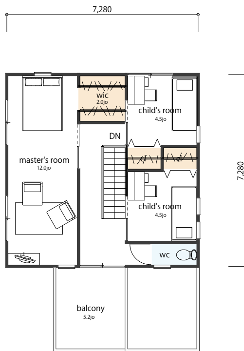
FLOOR PLAN 2F
