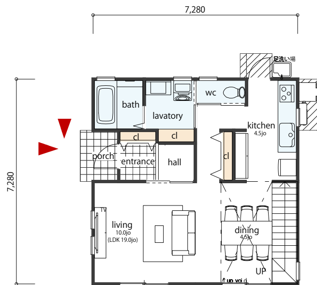
FLOOR PLAN 1F
