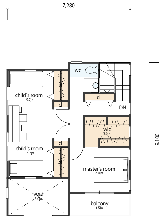
FLOOR PLAN 2F
