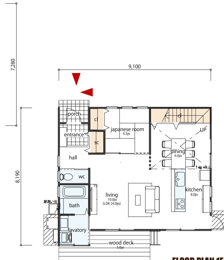
FLOOR PLAN 1F
