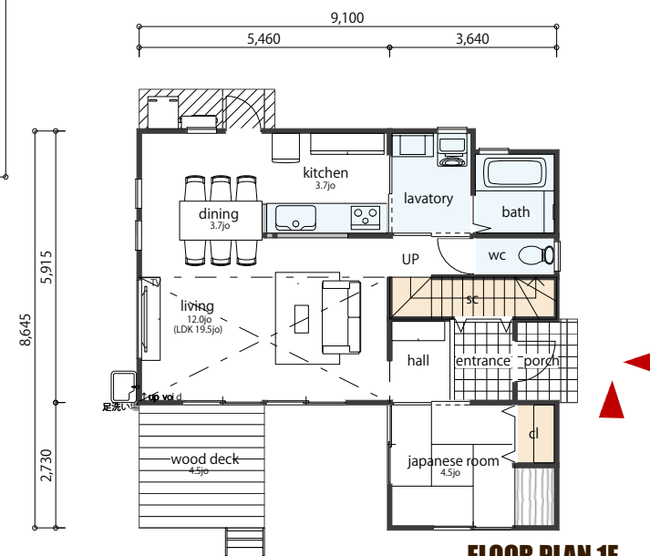
FLOOR PLAN 1F
