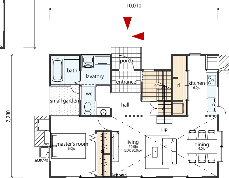
FLOOR PLAN 1F
